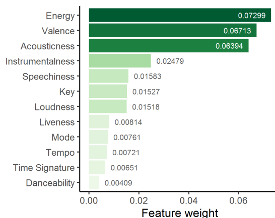
Figure 5. Influence of Spotify API features to separate songs among Russell's quadrants, according to Relief.
